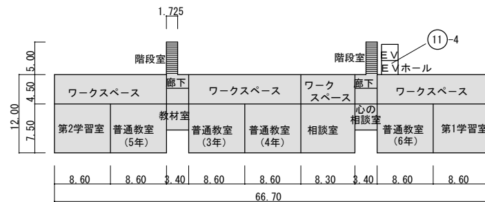
11-2 2階
