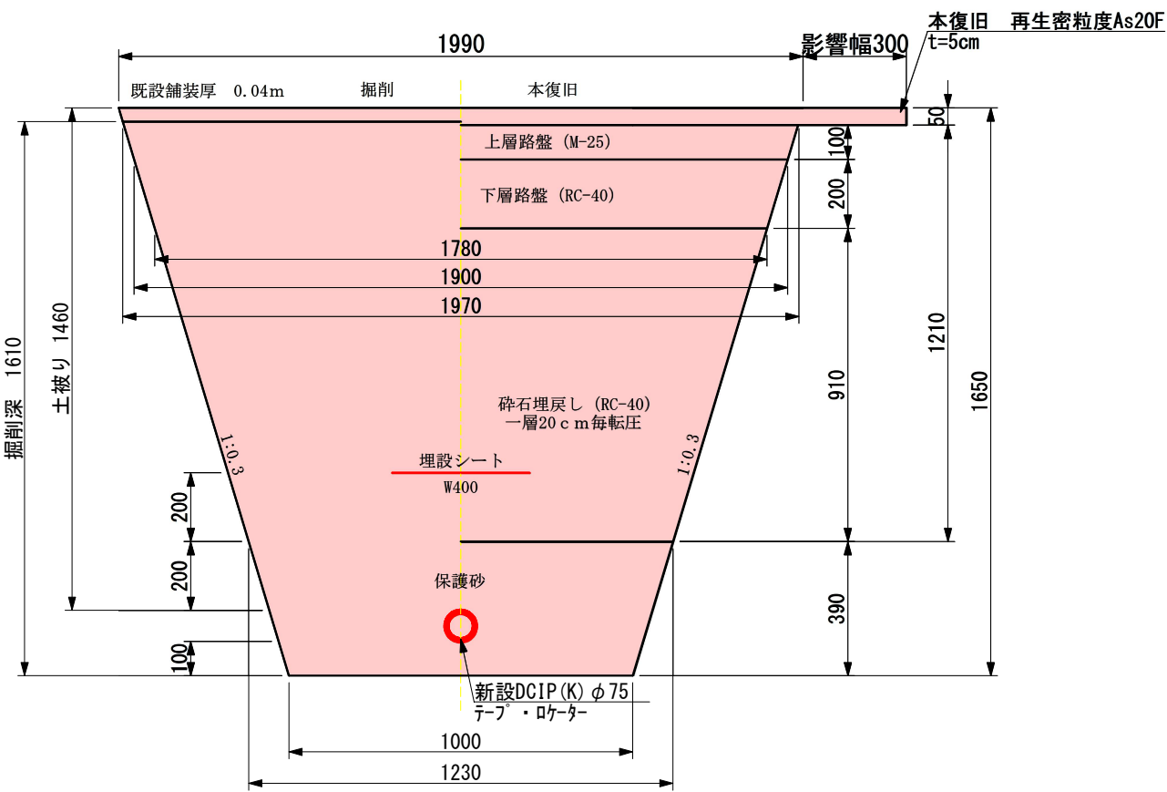
断面① L=4.0m
